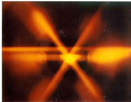
Figure 2: Cold sodium in an optical molasses at the intersection of six laser beams. Photo by Paul Lett (NIST group).
