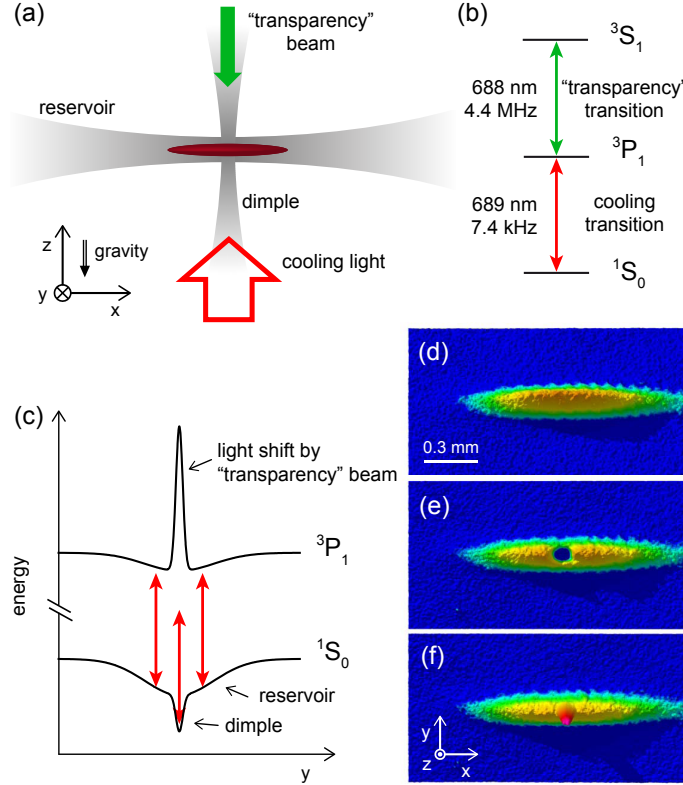
Figure 6: Transparency beam used in the strontium laser cooling to BEC experiment. The light shift in the trap center prevents photon reabsorption and allows very high densities. Figure from Ref. [10], copyright American Physical Society.
