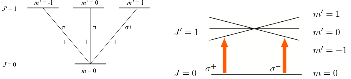
Figure 4: Left: coupling strength for the J = 0 \rightarrow J' = 1 transition. Right: Position-dependent coupling to the excited states, shifted by the magnetic field gradient (1D scheme).
